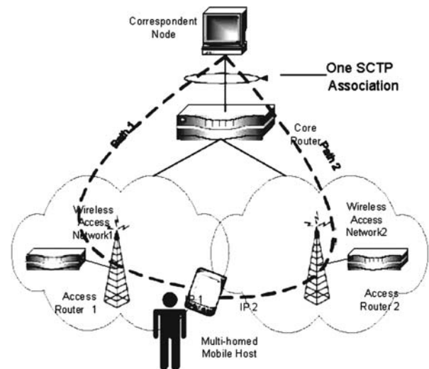
Fig. 1 A SCTP association featuring multi homing
