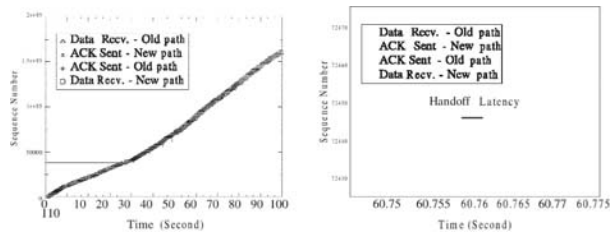
(a) Full range packet trace (b) Zoomed in view of the packet trace
