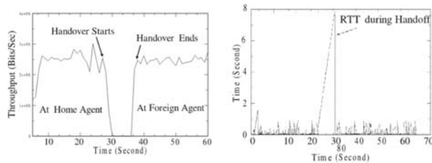
(a) Throughput (b) RTT Fig. 4 Throughput and RTT of Mobile IP handoff
