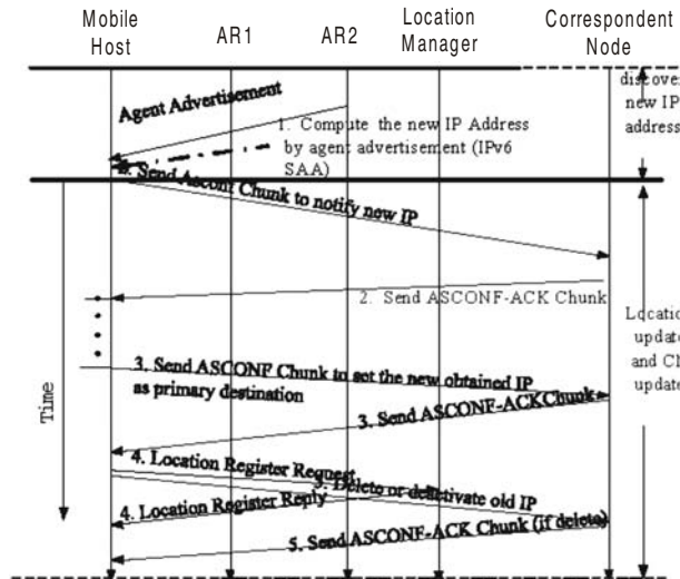
Fig. 2 Timeline of SIGMA
