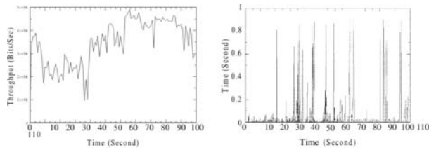
(a) Throughput (b) RTT Fig. 6 Throughput and RTT of SIGMA handoff
