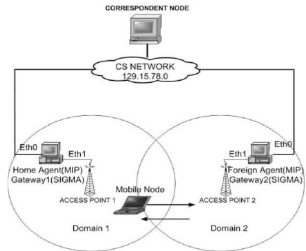
Fig. 3. SIGMA and Mobile IP testbed.
